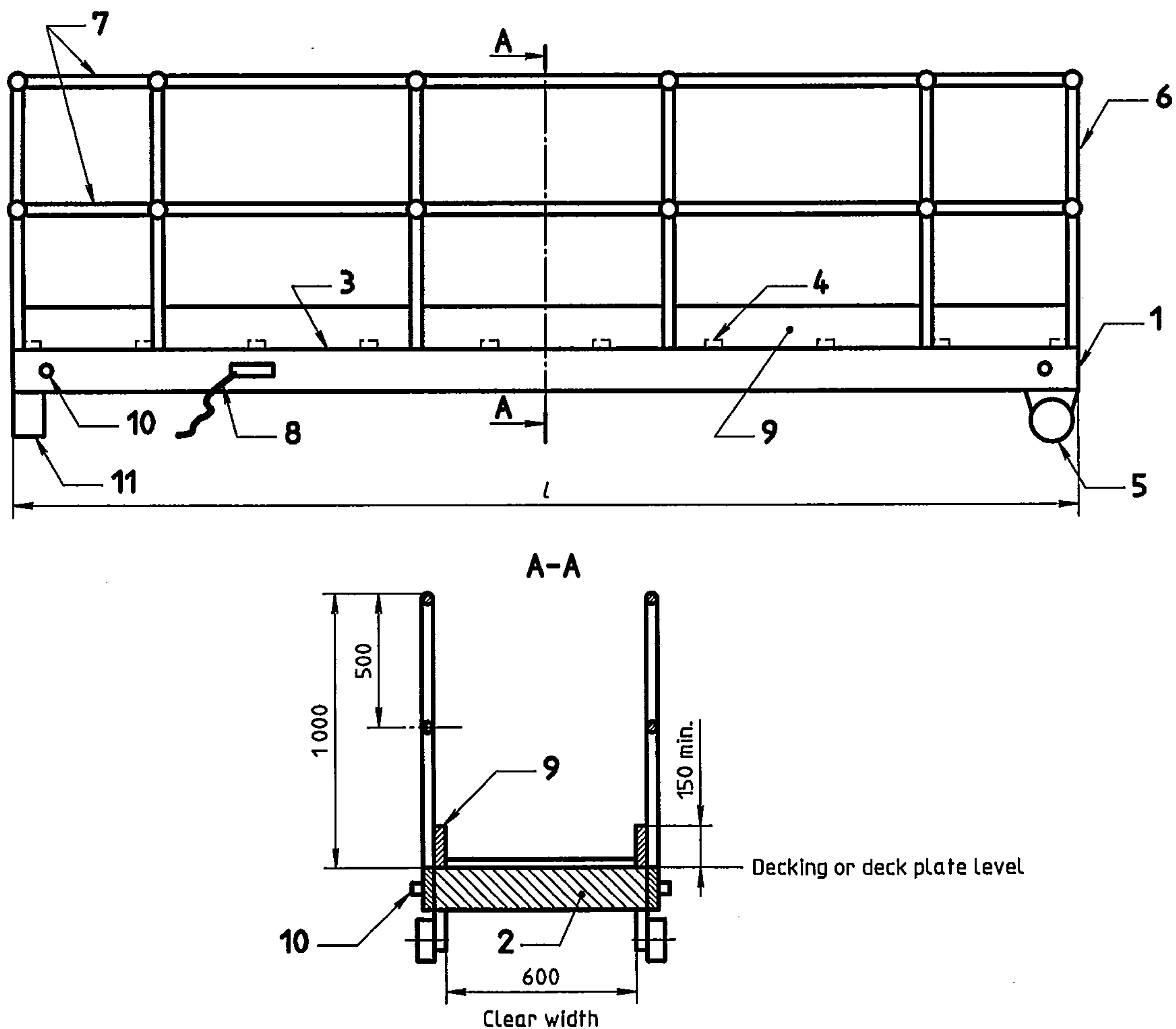
Figure 1 — General arrangement of a gangway (for item numbers, see table 1)
